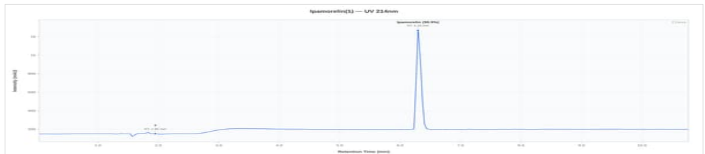
Ipamorelin 10mg - PX1IPA10-0021: UV Chromatogram
